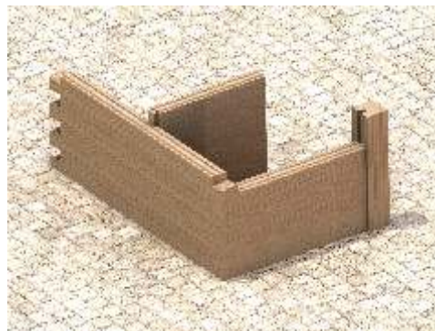
Corner of an external wall with a dovetail interlocking corner without remains.
